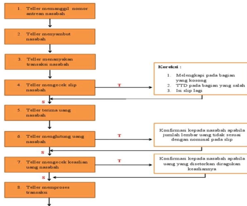
Gambar 1. Flow chart penerimaan kas
